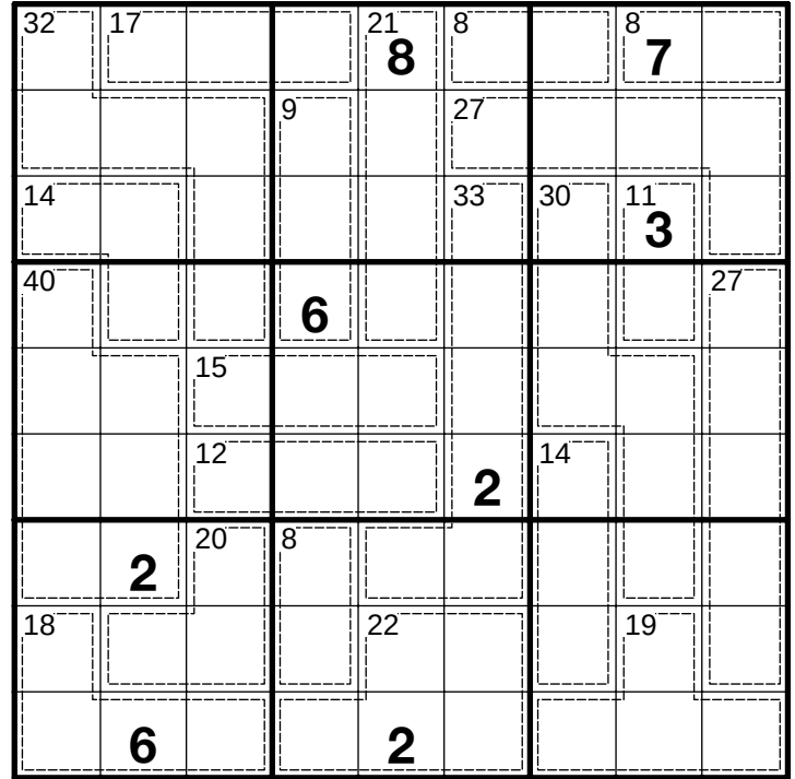
Killer Sudoku #662
