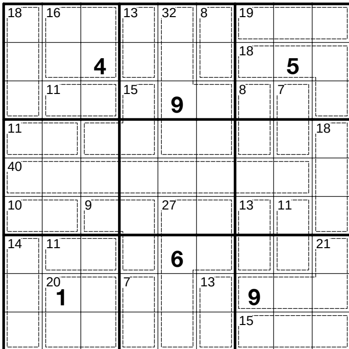
Killer Sudoku #715
