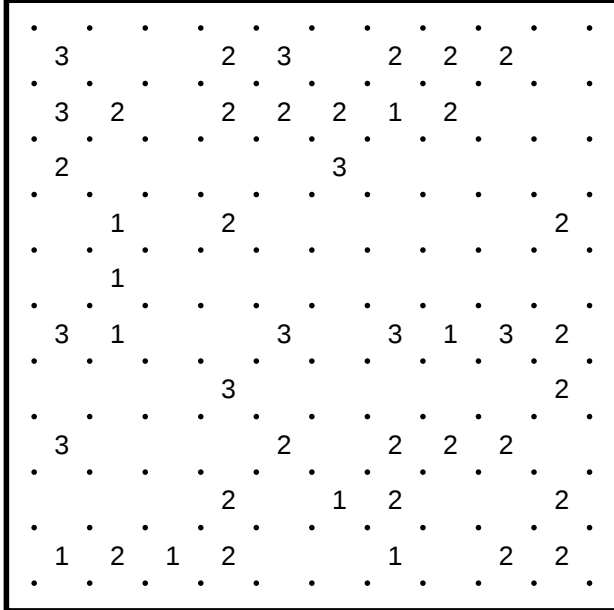
Slitherlink #3
