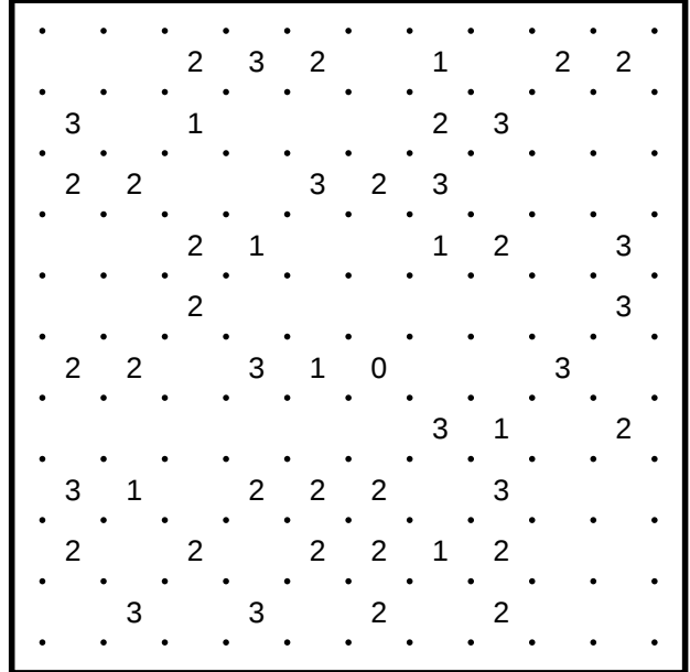
Slitherlink #4
