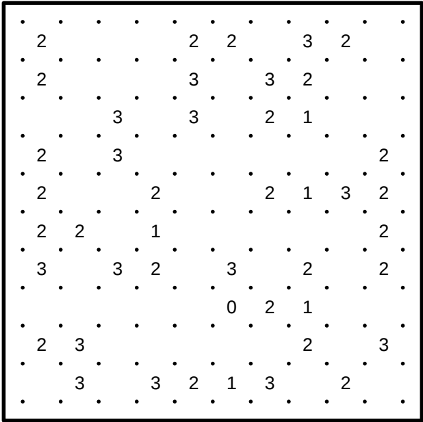
Slitherlink #9
