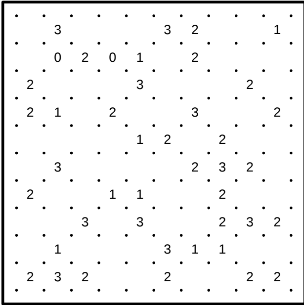
Slitherlink #10
