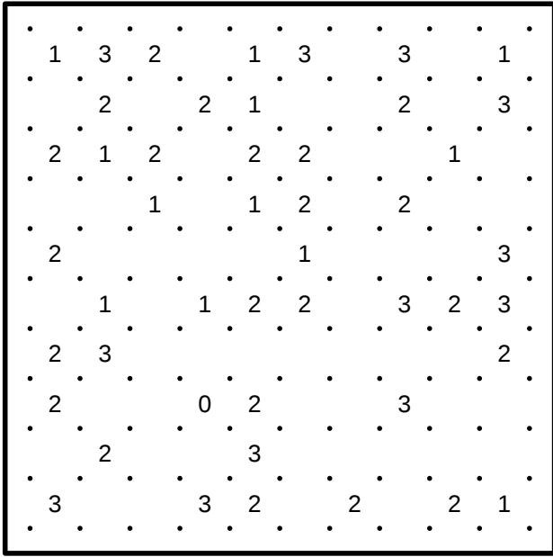
Slitherlink #12
