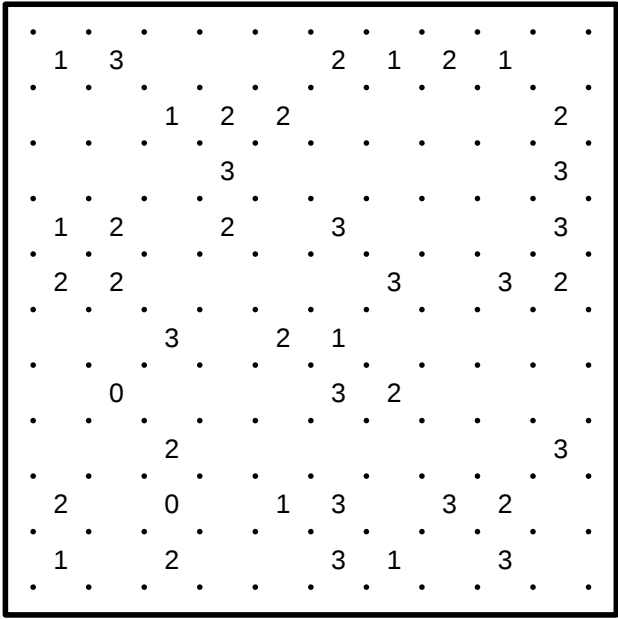
Slitherlink #11
