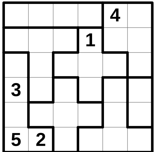
Suguru #8
