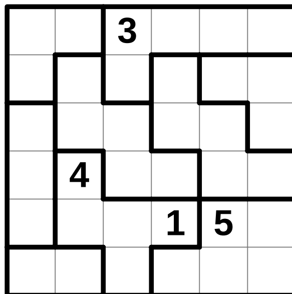
Suguru #4
