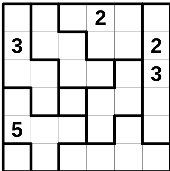
Suguru #3
