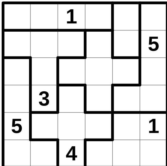
Suguru #1
