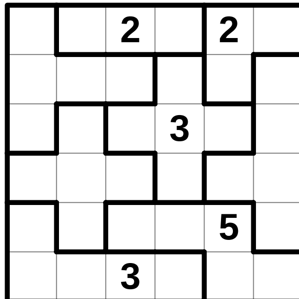
Suguru #2
